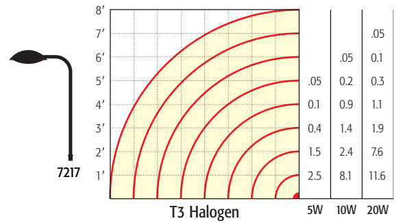
Horizontal Foot Candle Quarter Spread
