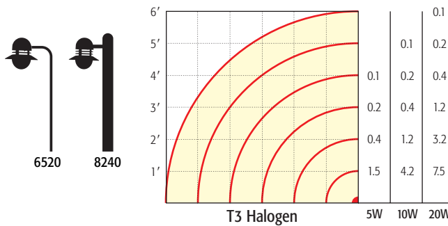
Horizontal Foot Candle Quarter Spread
