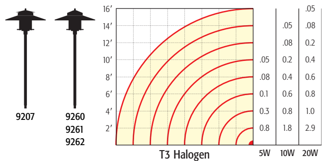
Horizontal Foot Candle Quarter Spread
