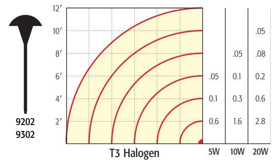
Horizontal Foot Candle Quarter Spread
