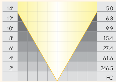
MR-16 LED: LN16-5.5-W-60-LED
