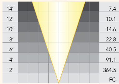
MR-16 LED: LN16-5.5-W-36-LED
