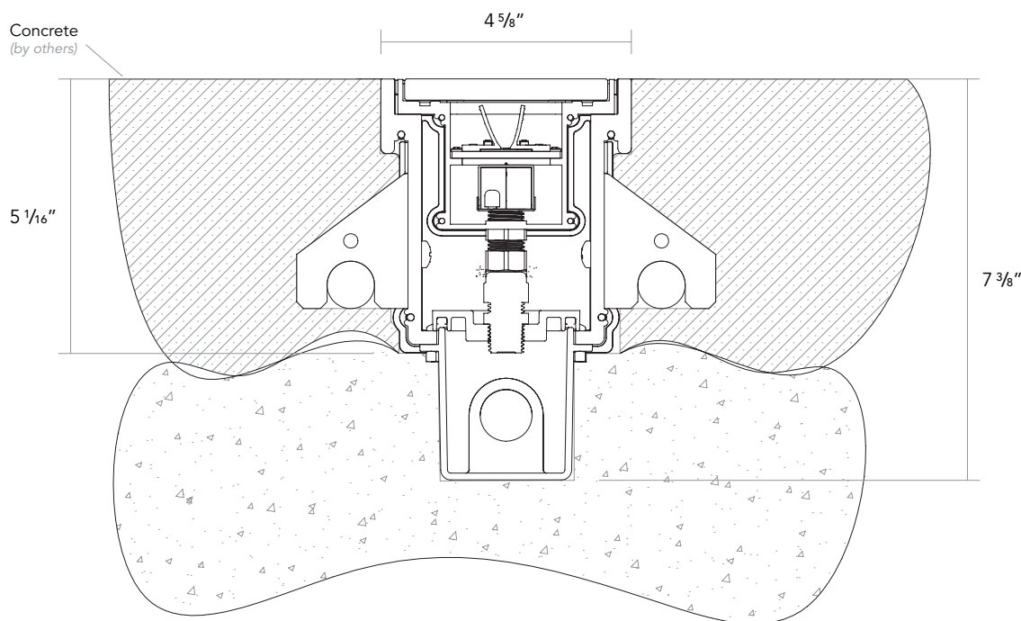
CONCRETE INSTALLATION
